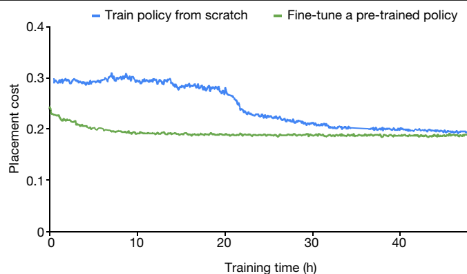
Fig. 4 | Convergence plots on Ariane RISC-V CPU. Placement cost of training a policy network from scratch versus fine-tuning a pre-trained policy network for a block of Ariane RISC-V CPU. Density weight was set to 0.1 and congestion weight to 0.
